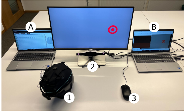
Figure 2: Arrangement of the multi-device multi-computer experiment. The brain-computer interface (1) is connected to the leftmost computer (A) which has a independent recording software (Unicorn Recorder). The eye-tracker (2) and the mouse (3) are connected to the rightmost computer (B). The recording software of the eye-tracker (Gazepoint Analysis), the mouse tracker (MouseCursorTracker Python library), and the stimulus presentation software (PsychoPy) are all running on computer B.
