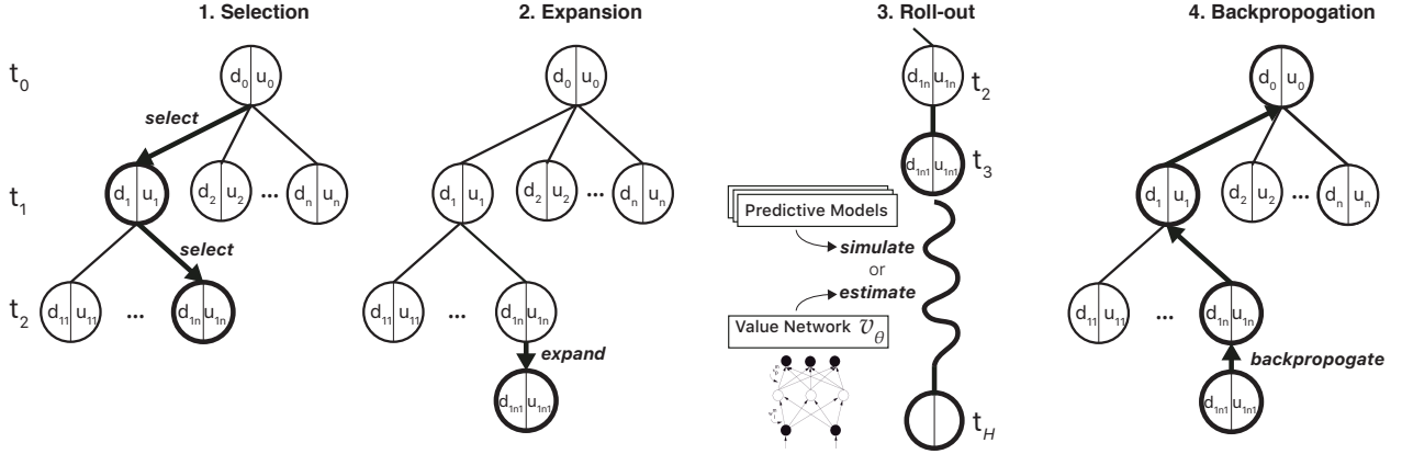
Figure 2: Model-based planning of adaptations using Monte-Carlo Tree Search (MCTS). Adaptations are selected using upper-confidence trees (UCT). After expanding a new node (adaptation), reward estimates are obtained through roll-outs, and backpropagated to the root node. The child with the highest value is picked as the next adaptation.
